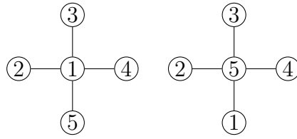
Figure 2.5: 132-representable (left) and non-132-representable (right) labelings of the same graph
