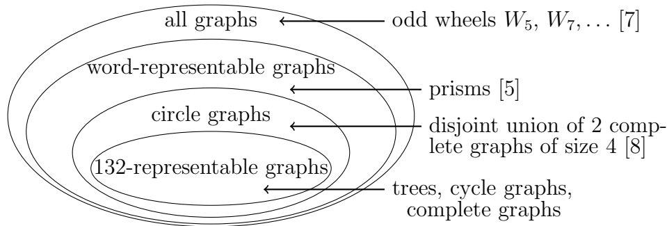
Figure 1.1: The place of 132-representable graphs in a hierarchy of graph classes
