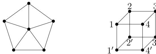
Figure 2.2: The wheel graph W_5 and the prism Pr_4
