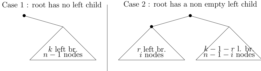
Figure 6: Counting binary trees along number of left branches
