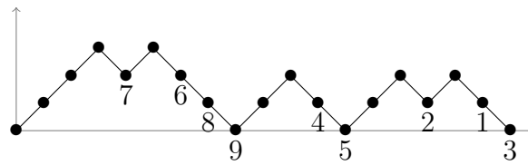
Figure 3: Dyck path obtained with the bijection by Krattenthaler over \sigma = 768945213 .
