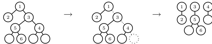
Figure 8: The bijection from \mathcal{T}_n^* to \mathcal{F}_n .
