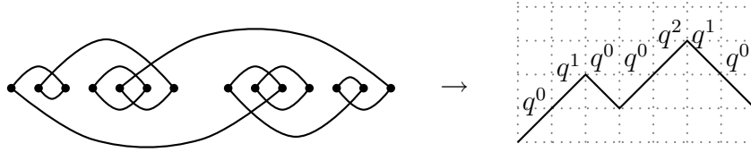
Figure 3: The bijection \Psi from \mathcal{C}_n to \mathcal{P}'_n in the case of \pi = 3, 4, -7, 2, 6, 1, 5 .
