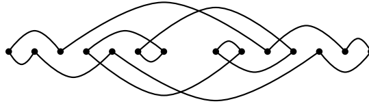
Figure 1: The arch diagram of \pi = 2, -4, 6, 1, -3, 7, 5 .
