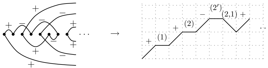
Figure 5: Construction of the bijection from the signed arch diagram of \pi \in \mathcal{C}_n to a labelled Motzkin path.
