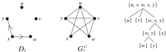
Figure 13: Example 5.8
