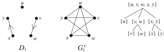
Figure 12: Example 5.7
