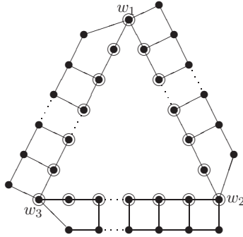
Figure 6: Graph G^k
