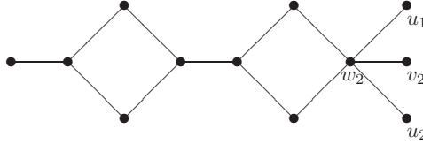
Figure 4: Graph G_2^2
