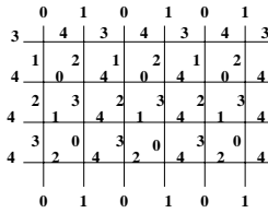
Figure 4: An AVD-coloring for TM_{4,6} .
