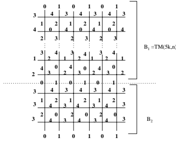
Figure 3: An AVD-coloring for TM_{5k+3,6} , with k \geq 1 .
