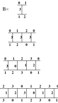
Figure 14: AVD-colorings for C_m \times P_2 , m = 3, 4, 8 .
