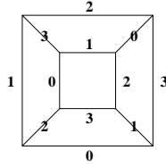
Figure 12: An AVD-coloring of H_3 .
