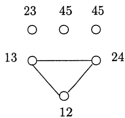
(a), nine edges omitted
