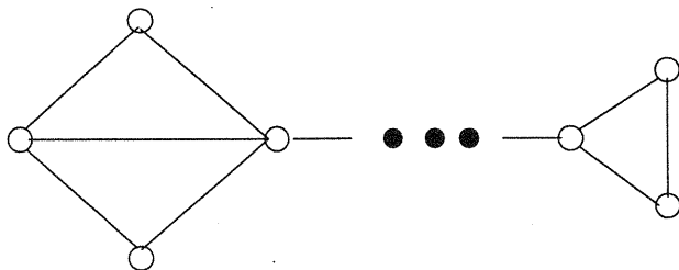
Figure 2: Theorem 4(j) (3)
