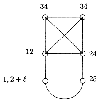
(b), with \ell = \text{ear length} ; in case \ell > 3 , the lists on the vertices between 25 and 1, 2 + \ell are \{k - 1, k\} , k = 6, \dots, 2 + \ell
