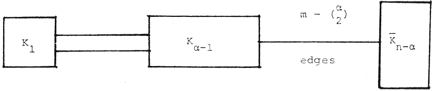
Figure 4.1 \mathcal{G}_1(n, m, \alpha)
