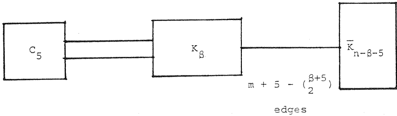
Figure 4.2 \mathcal{G}_2(n, m, \alpha)
