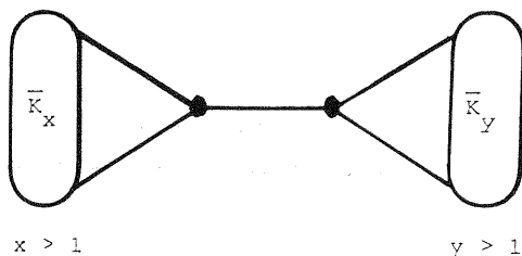
Figure 2.2 Double star
