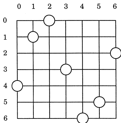
Figure 4.2 Compressed representation of covering of Figure 4.1
